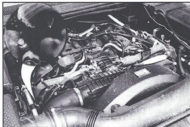
View of engine with top cover removed - right hand EGR valve shown in inset
