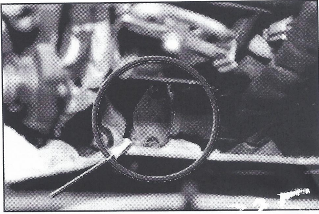
EGR valve blank fitted - indent arrowed!
